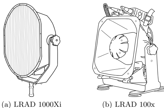
Figure 20.4: LRAD Models 12
